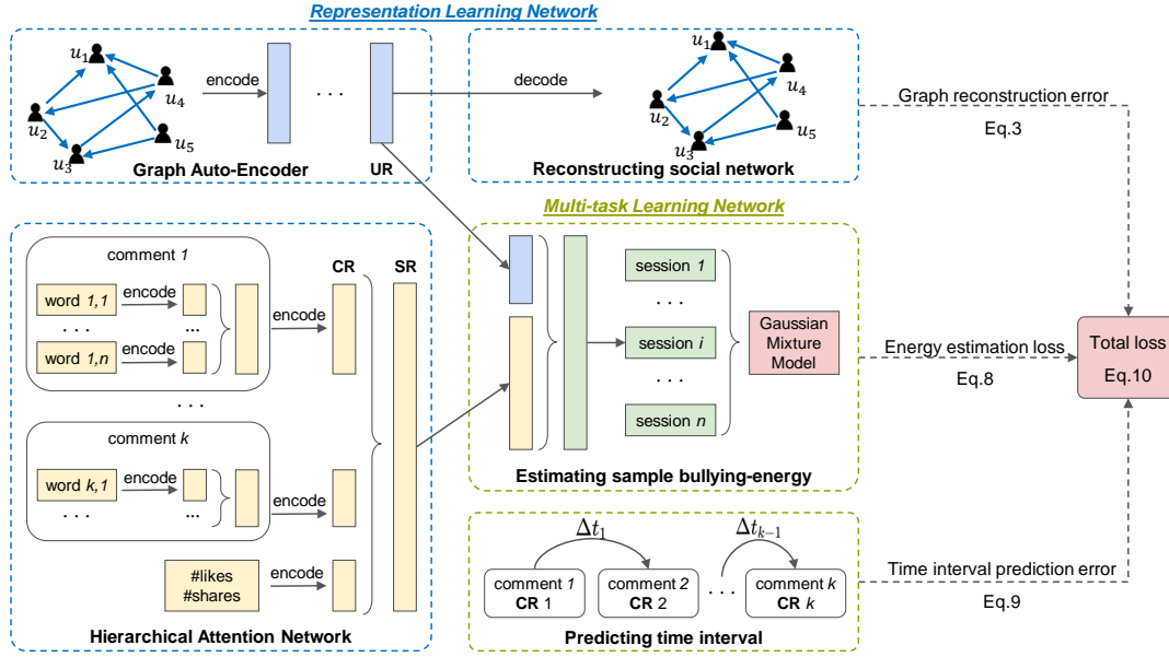
Figure 2: Overview of the proposed framework. UCD consists of two components: (1) The representation learning network (the blue dashed rectangles) constructs multi-modal representations of social media sessions (the green solid rectangles in the middle); (2) The multi-task learning network (the green dashed rectangles) that simultaneously estimates the energy/likelihood of input samples and predicts time intervals between comments. In particular, the representation learning network combines user (session owner) representation (UR) in Graph Auto-Encoder (top part) and social representation (SR) in Hierarchical Attention Network (HAN, bottom left) to form the session representation. The constructed session representation is the input of the sample bullying-energy estimation task. Meanwhile, the comment representations (CR) in HAN are fed into the time interval prediction task (bottom part). The overall loss comes from three sources: graph reconstruction error, energy estimation loss, and time interval prediction error. Best viewed in colors.
