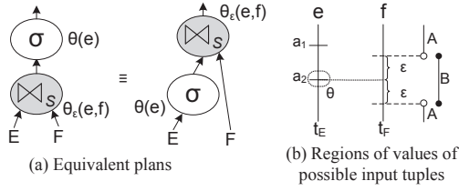
Fig. 21 Distribution of selection over \varepsilon -Join (R70)
