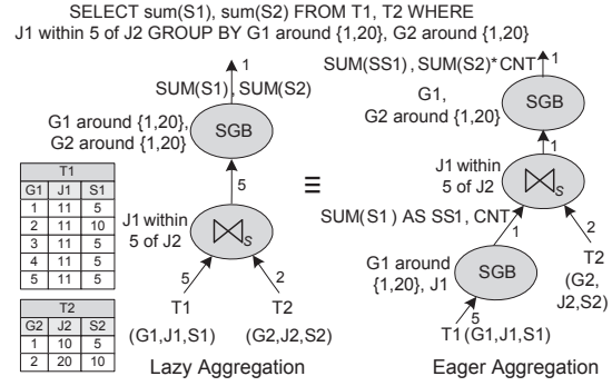
Fig. 31 Eager/Lazy aggregation with SGB and SJ
