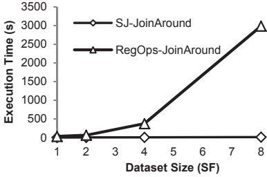
Fig. 41 Perf. of Join-Around while increasing dataset size
