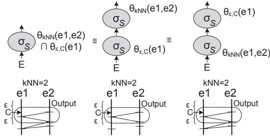
Fig. 17 Combining/separating kNN-Join and \varepsilon -Sel. (R23)
