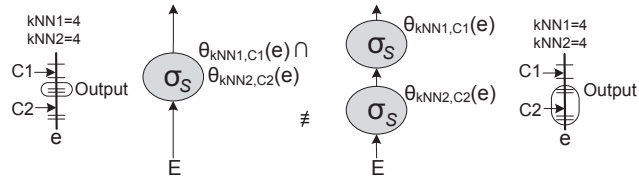
Fig. 12 Combining/separating kNN-Sel. and kNN-Sel. (R4)
