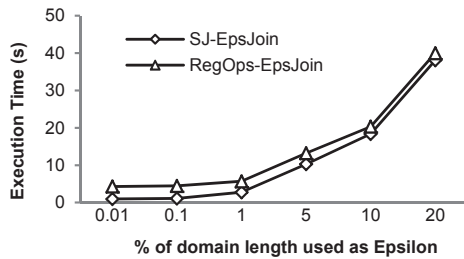
Fig. 42 Performance of \epsilon -Join while Increasing \epsilon
