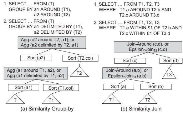
Fig. 38 Path/Plan trees with SGB and SJ operators
