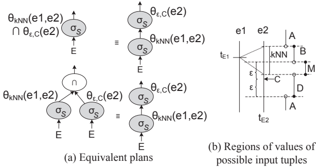
Fig. 18 Combining kNN-Join and \varepsilon -Sel. (R9) - proof
