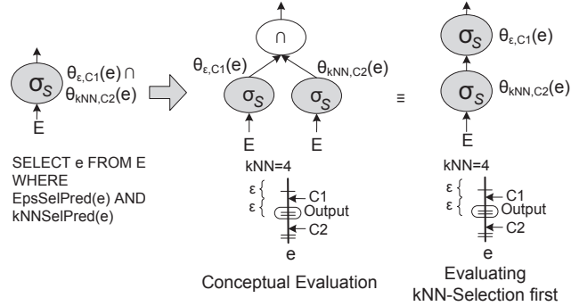
Fig. 6 Using the conceptual evaluation order
