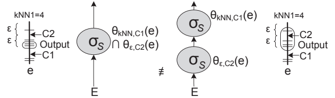
Fig. 11 Combining/separating kNN-Sel. and \varepsilon -Sel. (R3)
