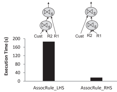
Fig. 43 Effectiveness of the associativity transformation
