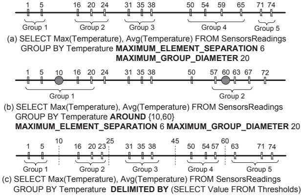
Fig. 1 Types of Similarity Group-by
