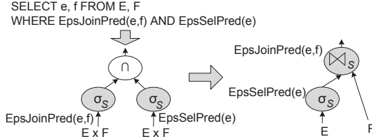
Fig. 32 Query with \varepsilon -Selection and \varepsilon -Join predicates
