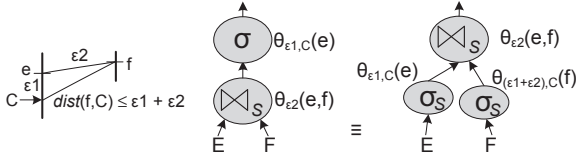
Fig. 28 Pushing \varepsilon -Selection predicate to an originally unrelated \varepsilon -Join operand (GR14)
