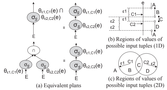
Fig. 13 Combining \varepsilon -Sel. and \varepsilon -Sel. (R1) - proof
