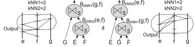
Fig. 26 Associativity of kNN-Join - when the attributes do not have a single direction: e \rightarrow f, f \leftarrow g (R107)
