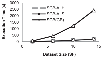
Fig. 40 Generating similarity groups with group-by vs. SGB
