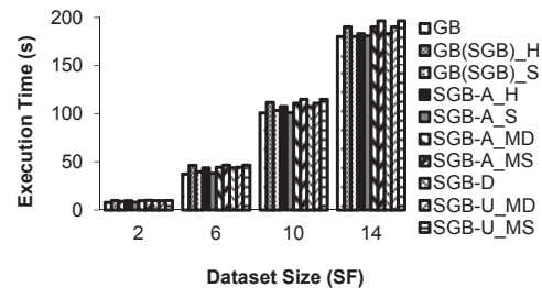
Fig. 39 Performance of SGB while increasing dataset size
