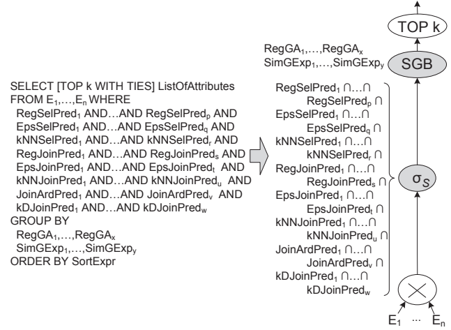
Fig. 4 Conceptual evaluation order of similarity queries
