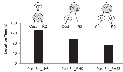
Fig. 44 Effectiveness of pushing selection below SJ
