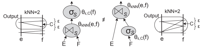
Fig. 23 Distribution of \varepsilon -Sel. over kNN-Join - when sel. is pushed below the inner relation (R89)
