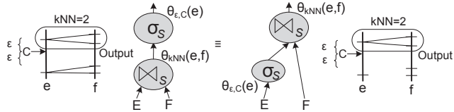
Fig. 22 Distribution of \varepsilon -Sel. over kNN-Join - when sel. is pushed below the outer relation (R88)
