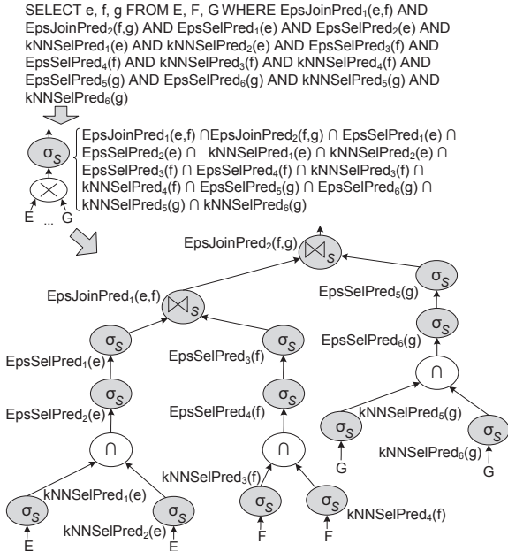
Fig. 35 Query with multiple \varepsilon -Join and sim. sel. predicates
