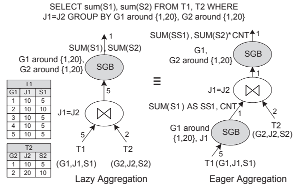
Fig. 29 Eager/Lazy aggregation with SGB and join
