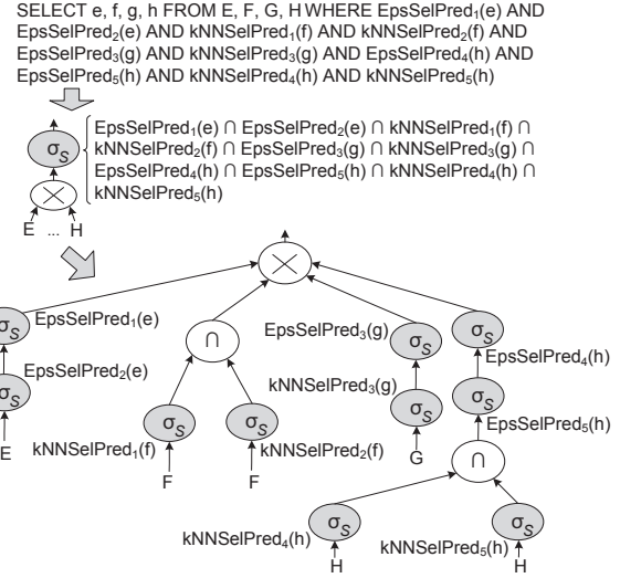
Fig. 34 Query with multiple sim. selection predicates
