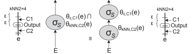
Fig. 10 Combining/separating \varepsilon -Sel. and kNN-Sel. (R2)
