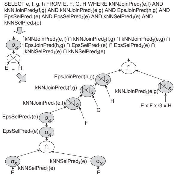
Fig. 37 Query with multiple sim. join and sel. predicates
