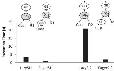
Fig. 46 Effectiveness of Lazy/Eager aggregations with SJ
