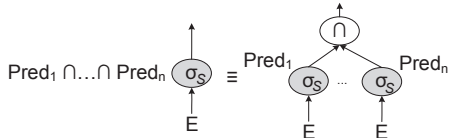
Fig. 5 Combining multiple similarity-aware predicates
