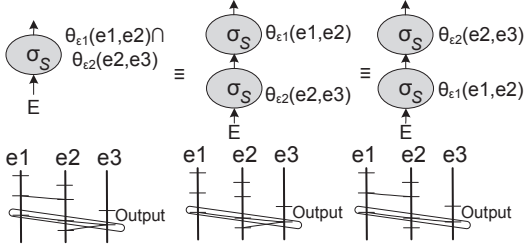
Fig. 20 Combining/separating two \varepsilon -Join predicates (R32)
