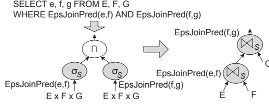
Fig. 33 Query with multiple \varepsilon -Join predicates
