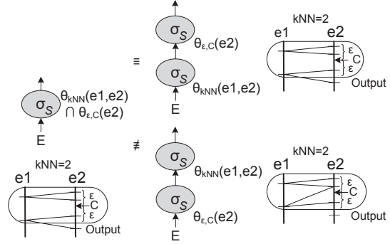
Fig. 16 Combining/separ. kNN-Join and \varepsilon -Sel. (R8, R9)
