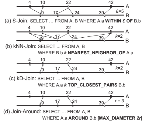
Fig. 2 Types of Similarity Join
