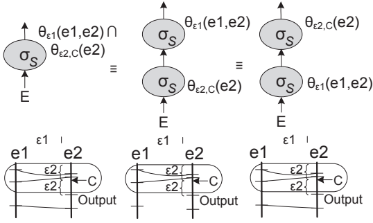
Fig. 15 Combining/separating \varepsilon -Join and \varepsilon -Sel. (R5)
